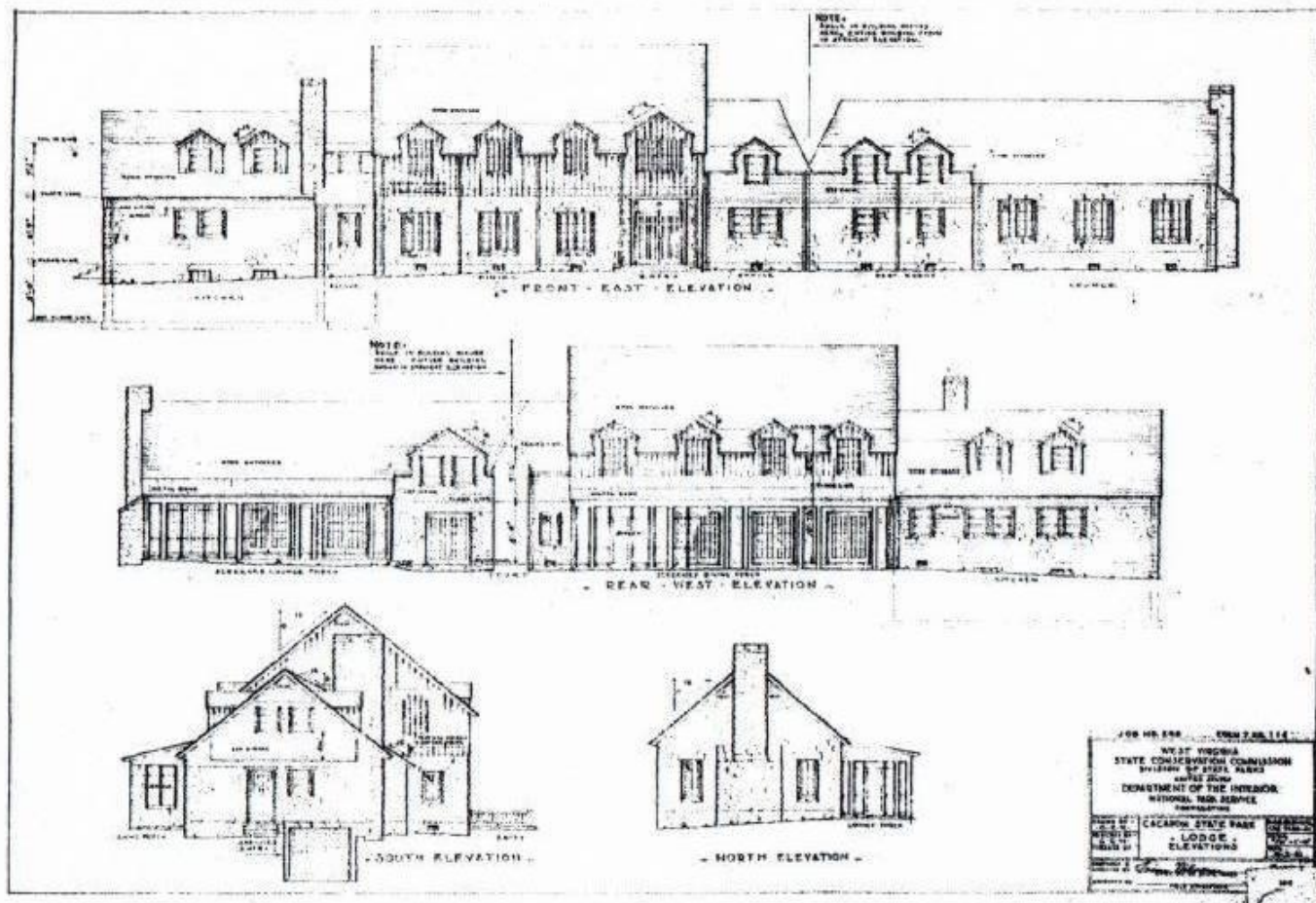
Figure 11: Cacapon State Park Lodge Elevations (United States Department of the Interior National Park Service Cooperating with West Virginia Conservation Commission). nd.
