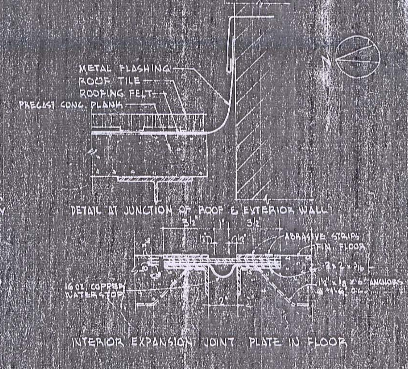
EXPANSION JOINT DETAILS SCALE 3/4" = 1'-0"
